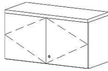
Swing Door Hanging Cabinet LD-0408W 800W x 380D x 400H LD-0409W 900W x 380D x 400H
