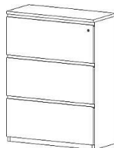
Lateral Filing Mid Cabinet LD-1208HF 800W x 400D x 1200H LD-1209HF 900W x 400D x 1200H LD-1210HF 1000W x 400D x 1200H
