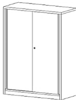
Sliding Door Mid Cabinet LD-1208S 800W x 400D x 1200H LD-1209S 900W x 400D x 1200H LD-1210S 1000W x 400D x 1200H
